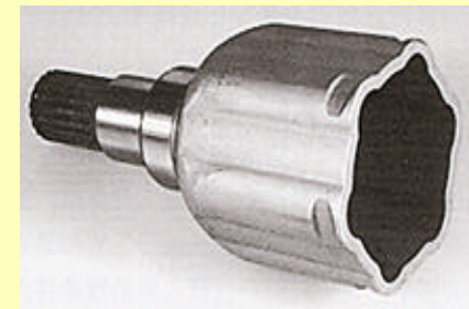
DOJプレス外輪 DOJ Outer Race with Stamped Cup
