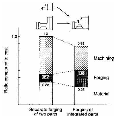
Fig.2 Forging cost of integrated transmission and synchronous gears [1]
